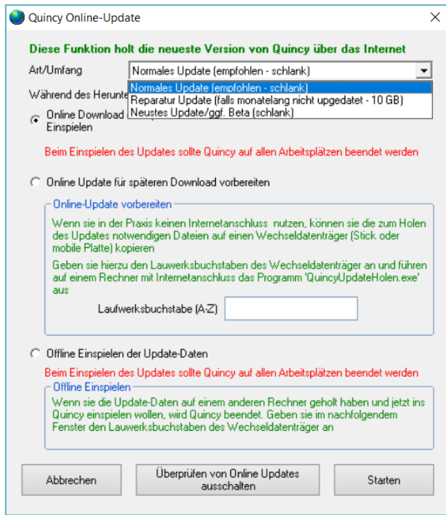
Abb. 3 Startfenster
