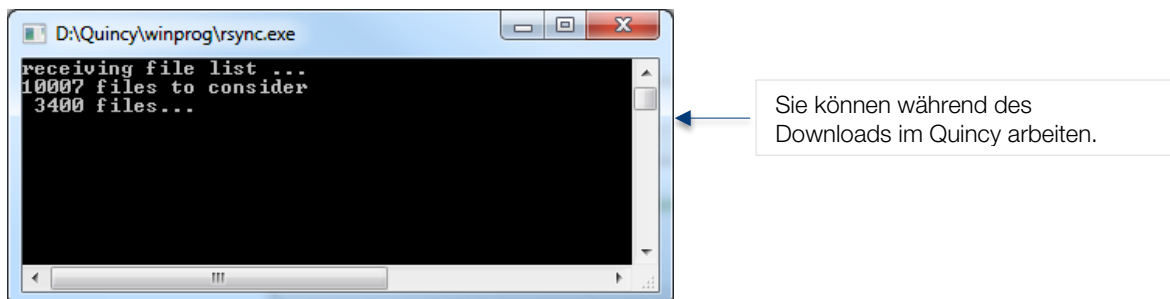
Abb. 6 Downloadfenster
